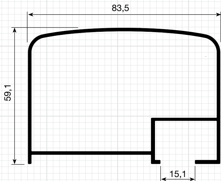
P-358 1,169 Kg/m
