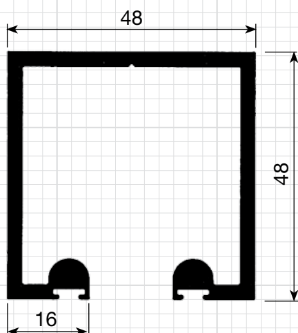
P-68 1,327 Kg/m
